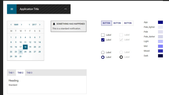
Example of reusable UI components from internal resources website
